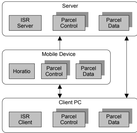
Figure 3: Control and Data Transfer in Horatio
