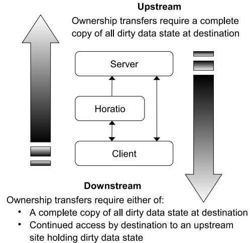
Figure 4: Rules for Ownership Transfer
