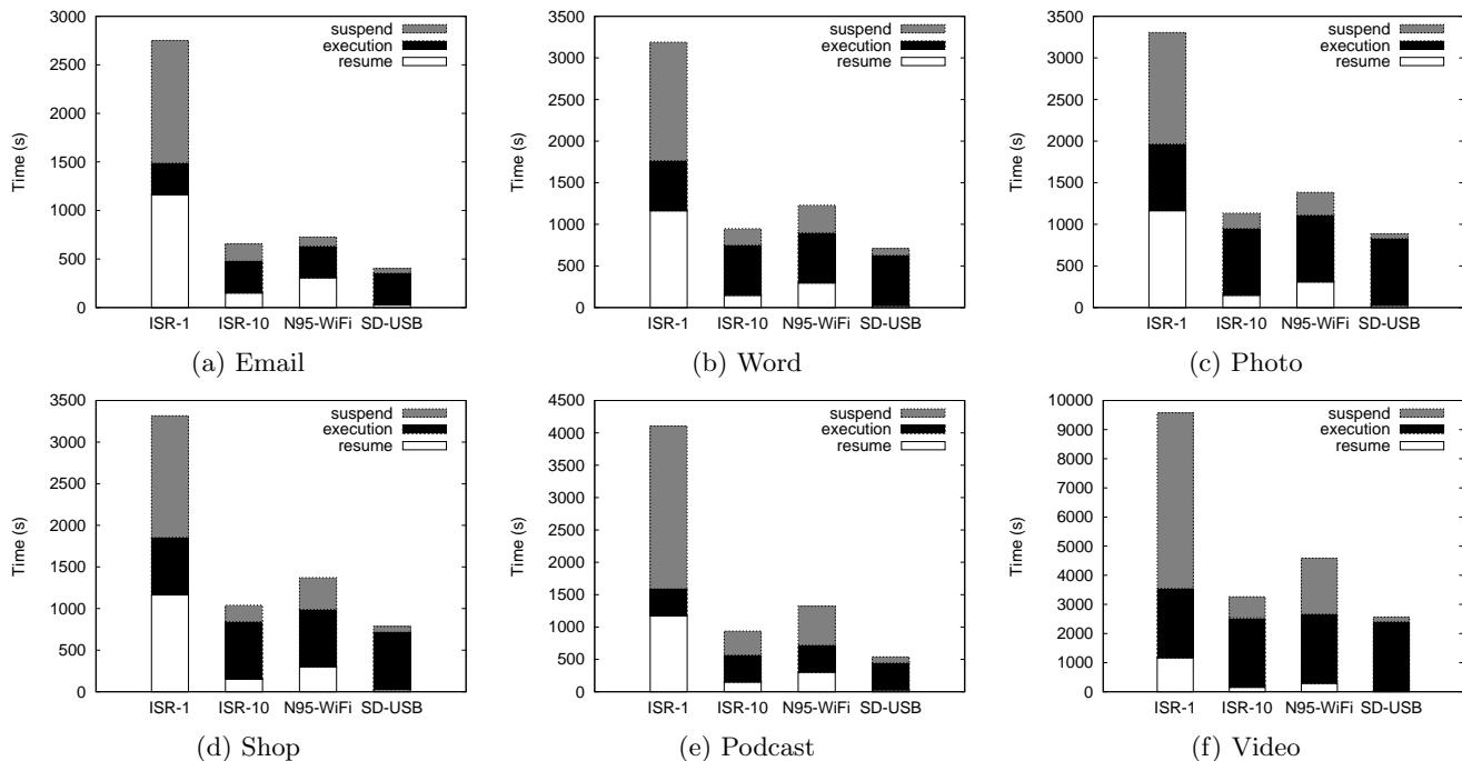
The figure shows that Horatio reduces suspend and resume times experienced by the user significantly over normal ISR. The ideal case is an all black bar. The ISR-1 and ISR-10 bars represent normal ISR with an emulated WAN link of 1Mbps and 10Mbps, respectively. Results are the mean of three measurements and standard deviations were below 19% in all cases. The scales of the graphs differ to improve the presentation.
