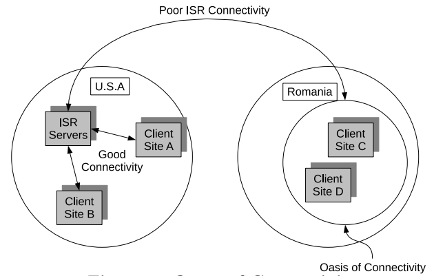
Figure 1: Oases of Connectivity
