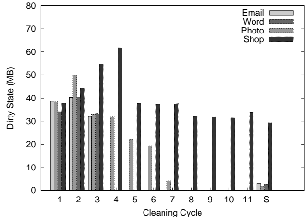
The distribution of state updates (in MB) for each workload during each periodic cleaning cycle. A cleaning cycle starts approximately one minute after the end of the preceding cycle. Suspend time is marked by an “S” on the horizontal axis.
