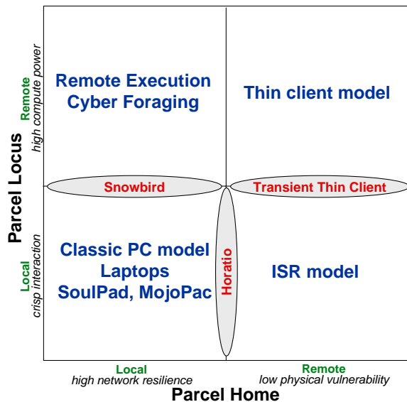
Figure 2: Separating Parcel Storage and Execution
